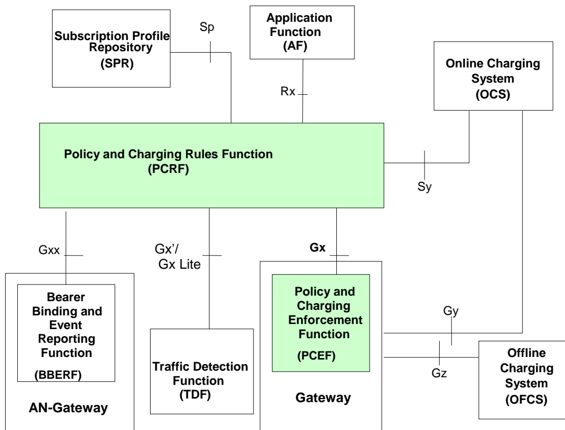
Figure 58 - Overall PCC logical architecture (non-roaming)
