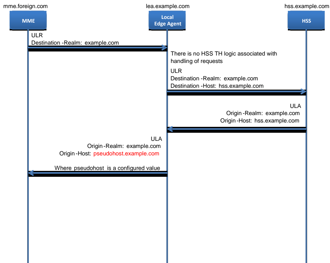
Figure 50 - S6a/S6d HSS Topology Hiding - ULR Message Flow
