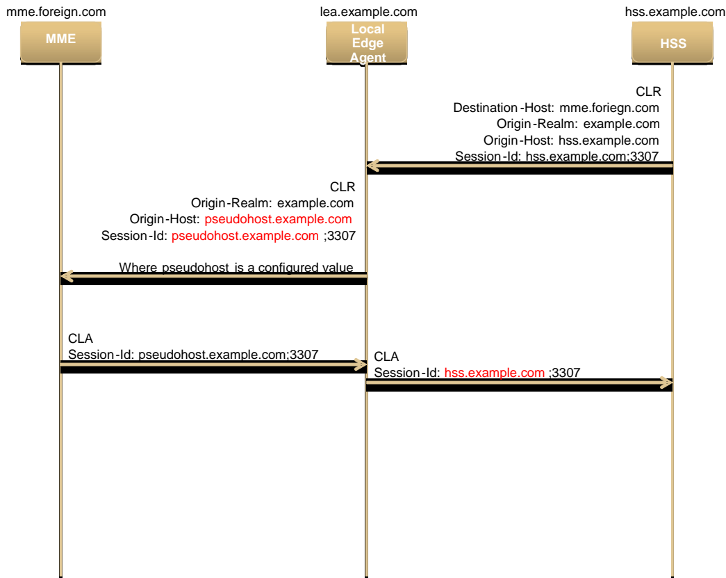
Figure 51 - S6a/S6d HSS Topology Hiding CLR Message Flow
