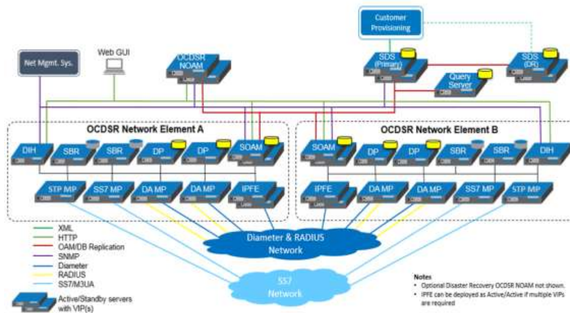
Figure 5 - DSR 8.x Architecture
