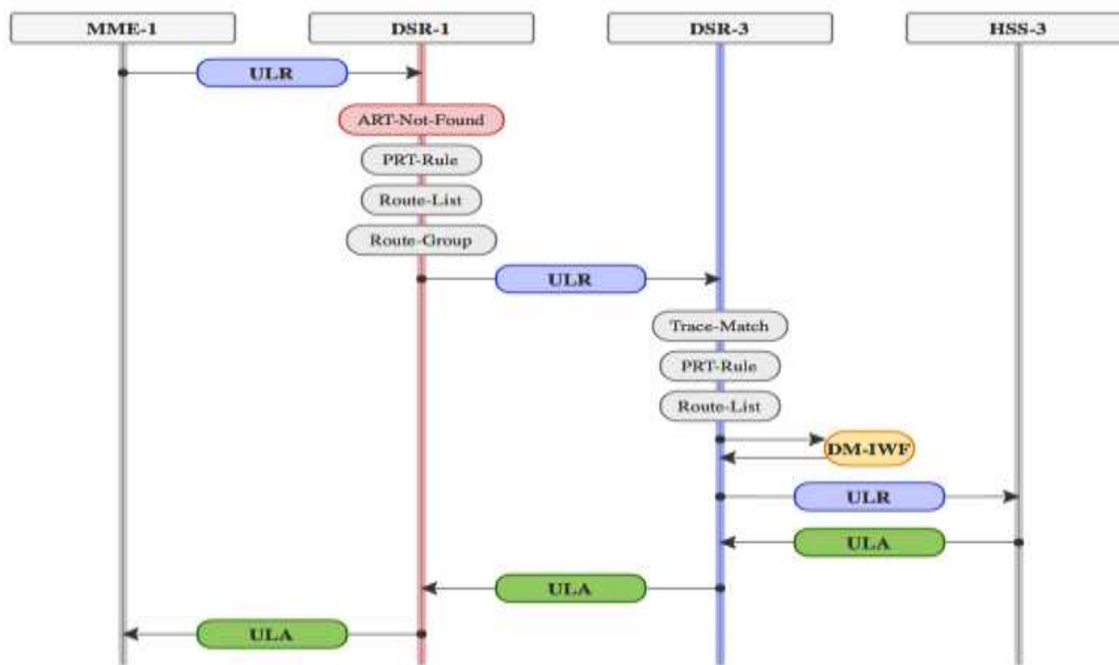
Figure 70 – Message Flow for Network Wide Trace
