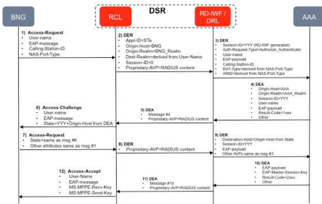
Figure 47 - RADIUS->Diameter IWF for Authentication
